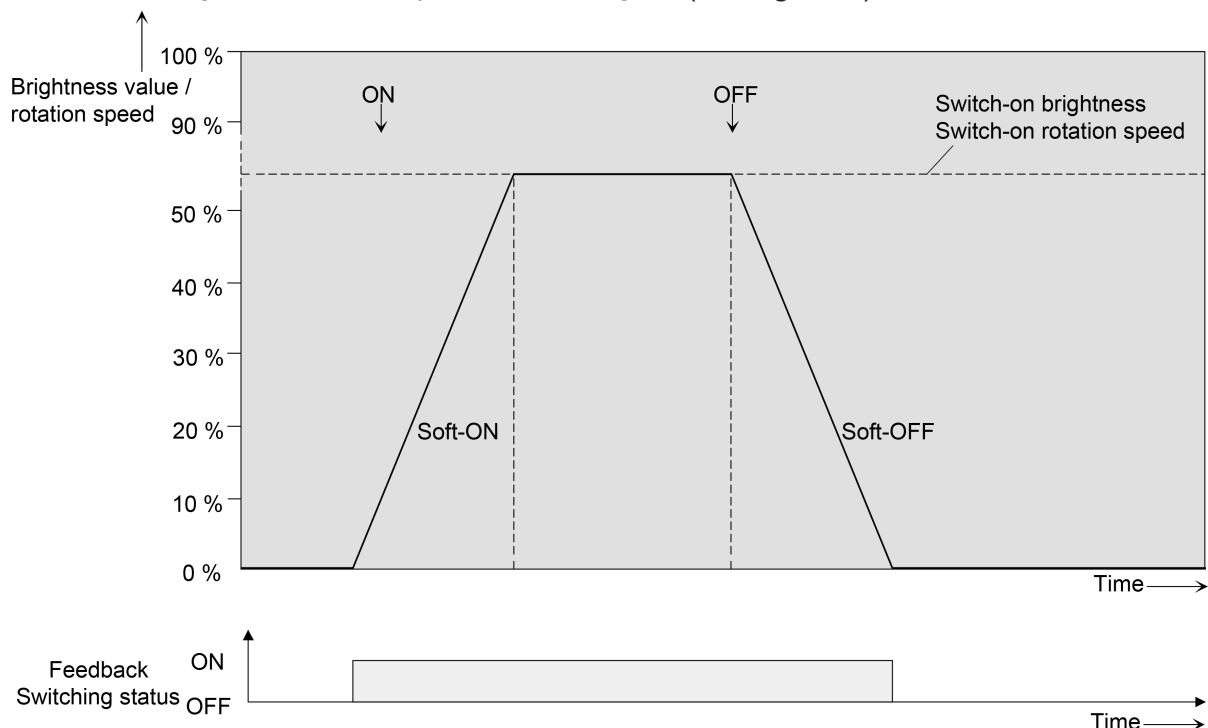
Image 8: Dimming behaviour of the soft ON/OFF functions (as an example)
