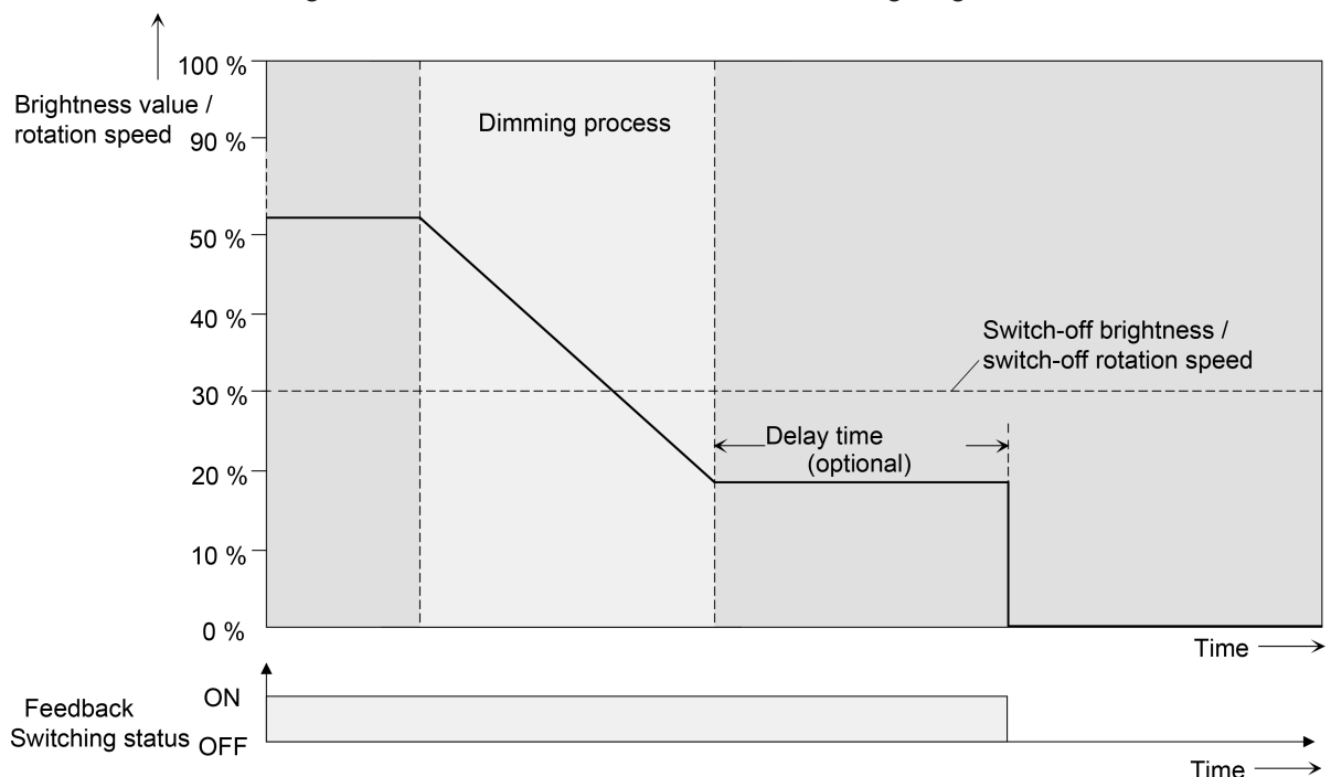
Image 9: Dimming and switching behaviour of the automatic switch-off function
