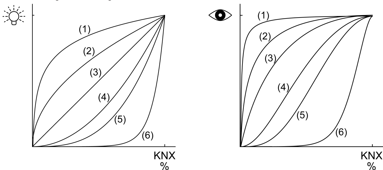
Image 1: Dimming characteristics in the value range
