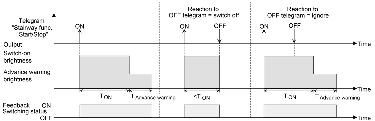
Image 12: Switch-off behaviour of the staircase function without soft functions
