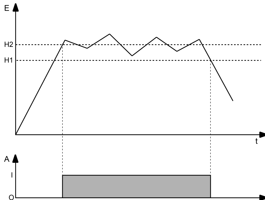
Image 39: Example of a hysteresis evaluation by upper and lower threshold value.
