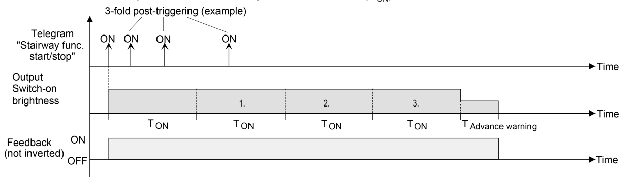
Image 18: Time extension of the staircase function
