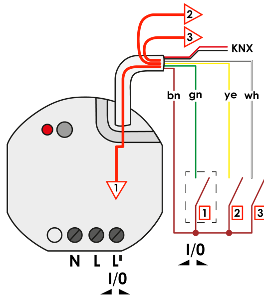
Image 22: Functioning of inputs when controlling the internal dimming output as single-area operation
