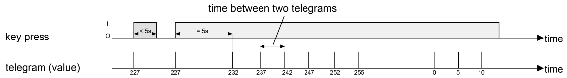
Image 28: Example of value adjustment with value range overflow
