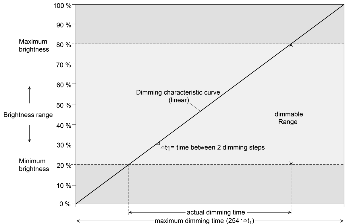
Image 3: Linear characteristic dimming curve as an example with minimum brightness > 0 % and maximum brightness
