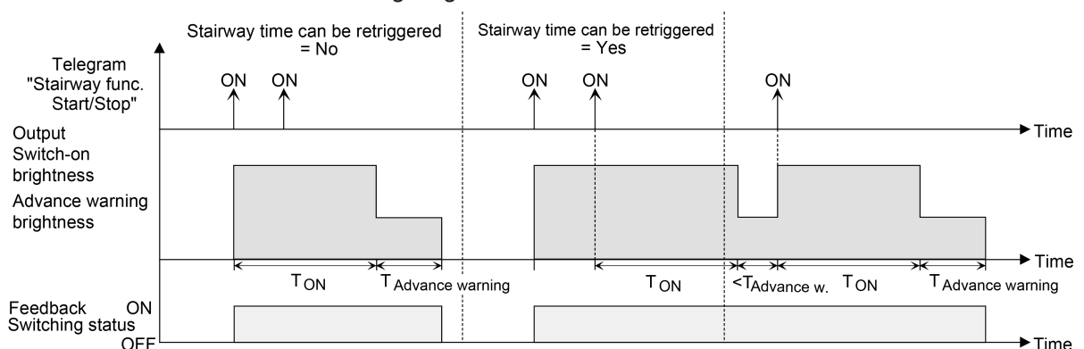
Image 10: Switch-on behaviour of the staircase function without soft functions
