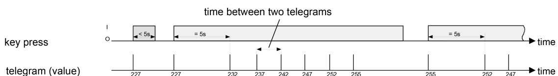
Image 27: Example of value adjustment without value range overflow
