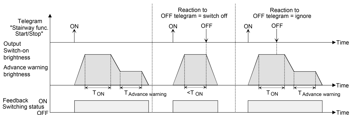
Image 13: Switch-off behaviour of the staircase function with soft functions (as an example with minimum brightness = 0 %)
