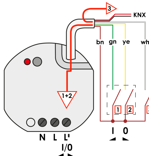
Image 21: Functioning of the inputs when controlling the internal dimming output as dual-area operation
