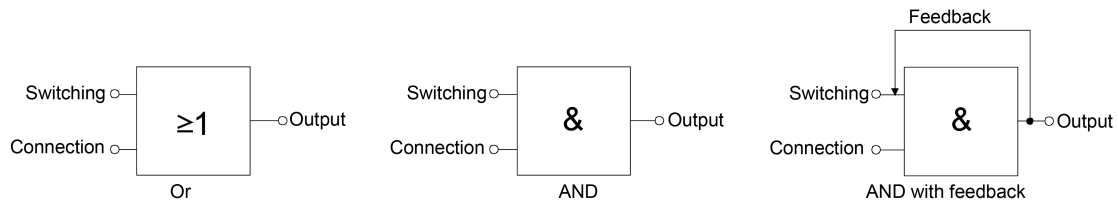
Image 19: Logic operation types of the logic operation function
