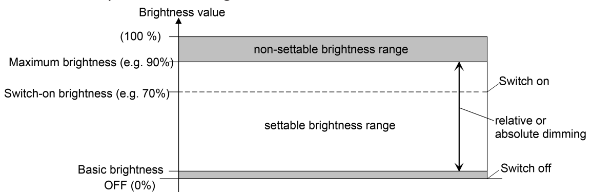
Image 6: Example of a brightness range with basic brightness
