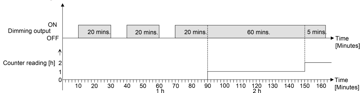
Image 20: Function of the operating hours counter (using the example of counted hours)
