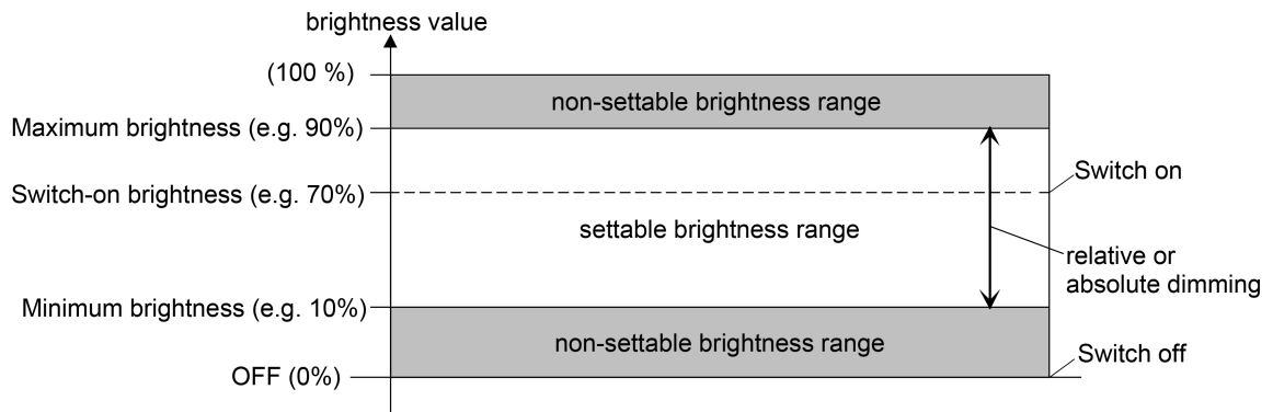
Image 7: Example of a brightness range with minimum brightness
