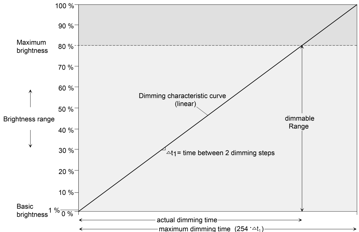
Image 2: Linear dimming characteristic as an example with basic brightness and maximum brightness
