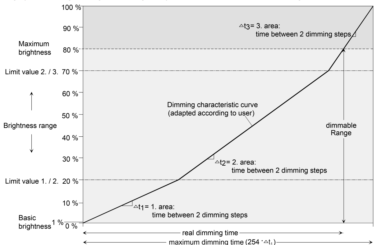
Image 4: User-defined dimming characteristic as an example with basic brightness and maximum brightness
