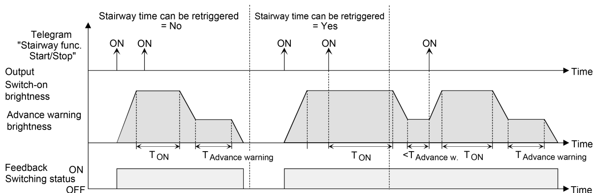
Image 11: Switch-on behaviour of the staircase function with soft functions (as an example with minimum brightness = 0 %)
