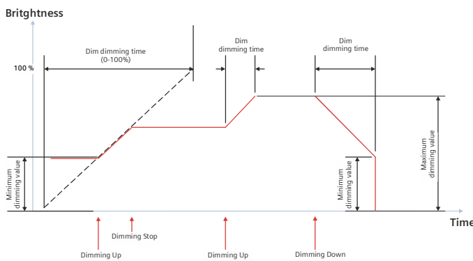
Dimming by dimming object (switch-off possible)
