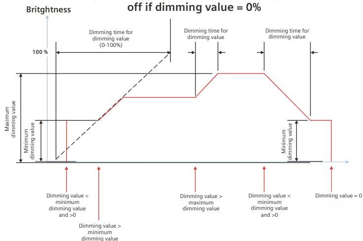
Switching via dimming value: on if dimming value > 0%, off if dimming value = 0%
