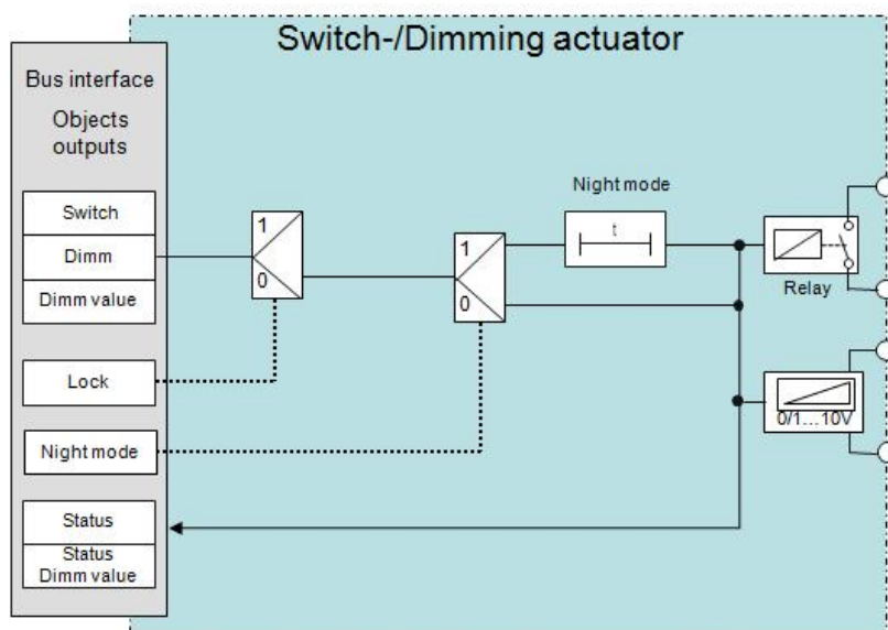
Schematic design of a dimming actuator channel
