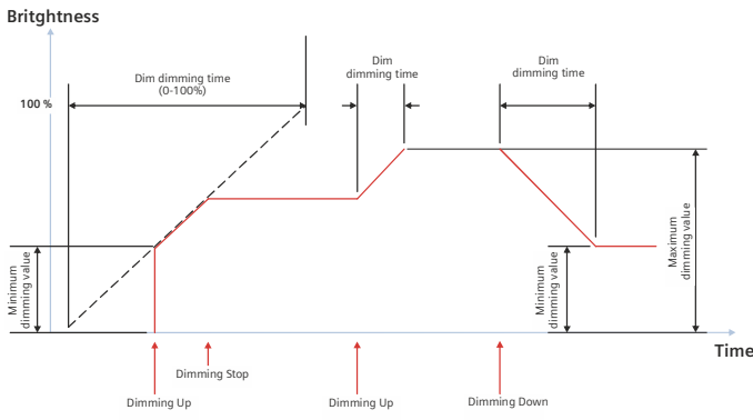
Dimming by dimming object (switch-on possible)
