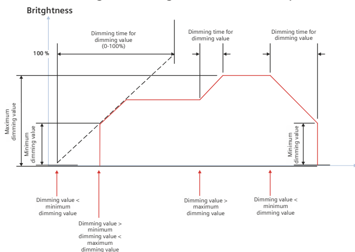
Switching via dimming value: switch-on/off possible
