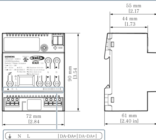
Fig. 10: Dimensions
