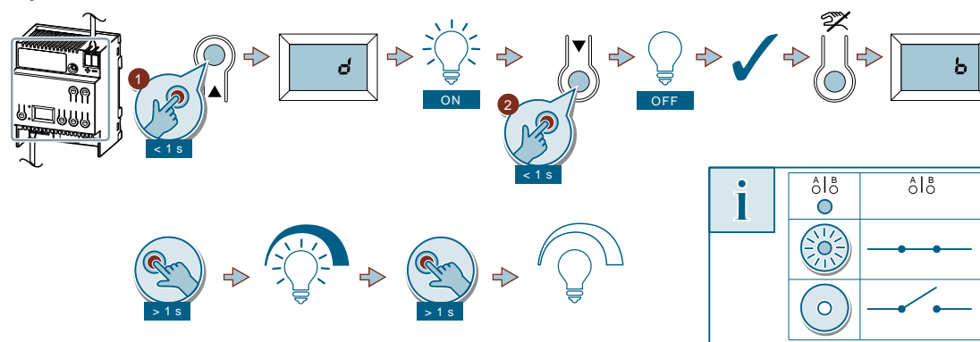
Fig. 8: Operation in direct mode
