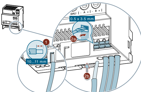
Fig. 5: Connecting DALI
