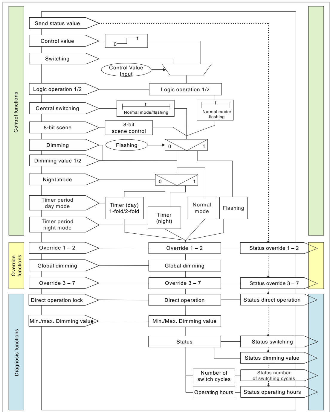
Fig. 1: Schematic design of a dimming channel
