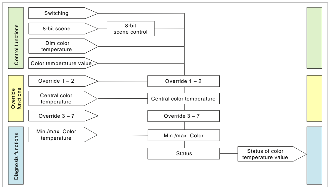
Fig. 2: Flow chart for color temperature control
