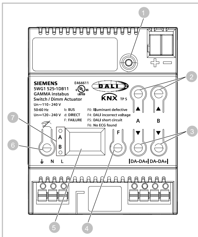
Fig. 3: User interface with operating and display elements
