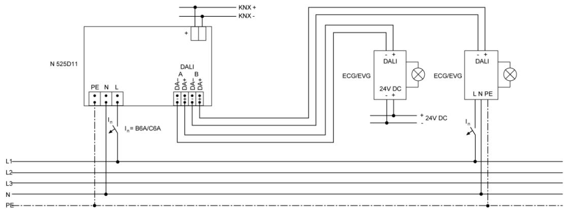
Fig. 11: Connection example
