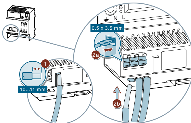
Fig. 4: Connecting the power supply
